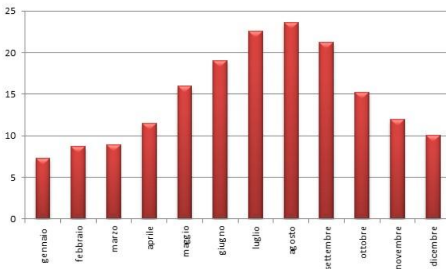
Figura 22 – Temperature medie mensili registrate (°C) – 2020
